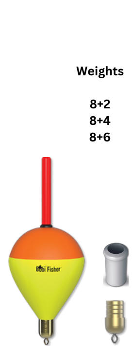
Model: TP 15 PRODUCT INFORMATION: Foam Float with brass weight and starlight antenna.
