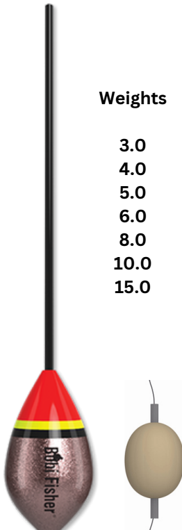
Model: BF 223 PRODUCT INFORMATION: Balsa Float with brass weight.
